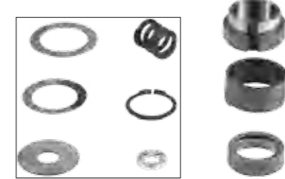
22253102 AYAR MEKANİZMA PUL SEKMAN TAKIMI / CALIPER ADJUSTING MECHANISM WASHER & RING SET
