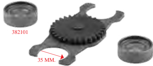
22311114 DİŞLİ SABİTLEME SAC VE TAPA TAKIMI LOCKING SHIM & SLOT SET
