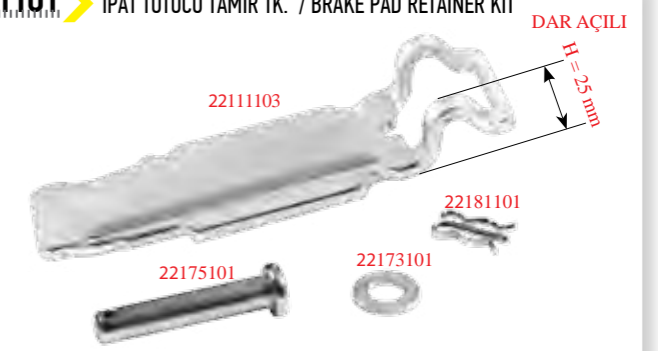
22111101 İPAT TUTUCU TAMİR TK. / BRAKE PAD RETAINER KIT
