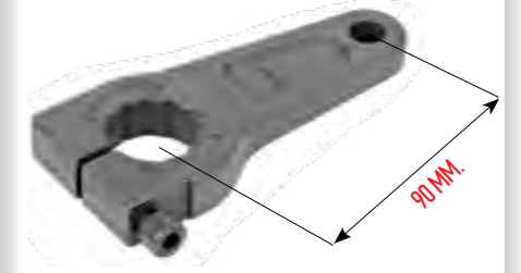
22314103 KALİPER SAFT LEVYESİ CALIPER SHAFT LEVER
