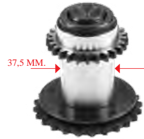
22303407 AYAR DIŞLİSİ -R CALIPER ADJUSTING GEAR - R -
