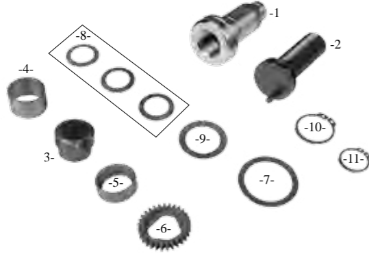
22202116 AYAR MEKANİZMASI PİMLİ CALIPER ADJUSTING MECHANISM (W/PIN)
