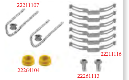
22211103 İPAT TUTUCU TAMİR TK. BRAKE PAD RETAINER KIT
