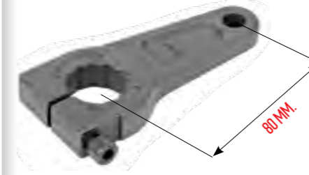
22314102 KALİPER SAFT LEVYESİ CALIPER SHAFT LEVER
